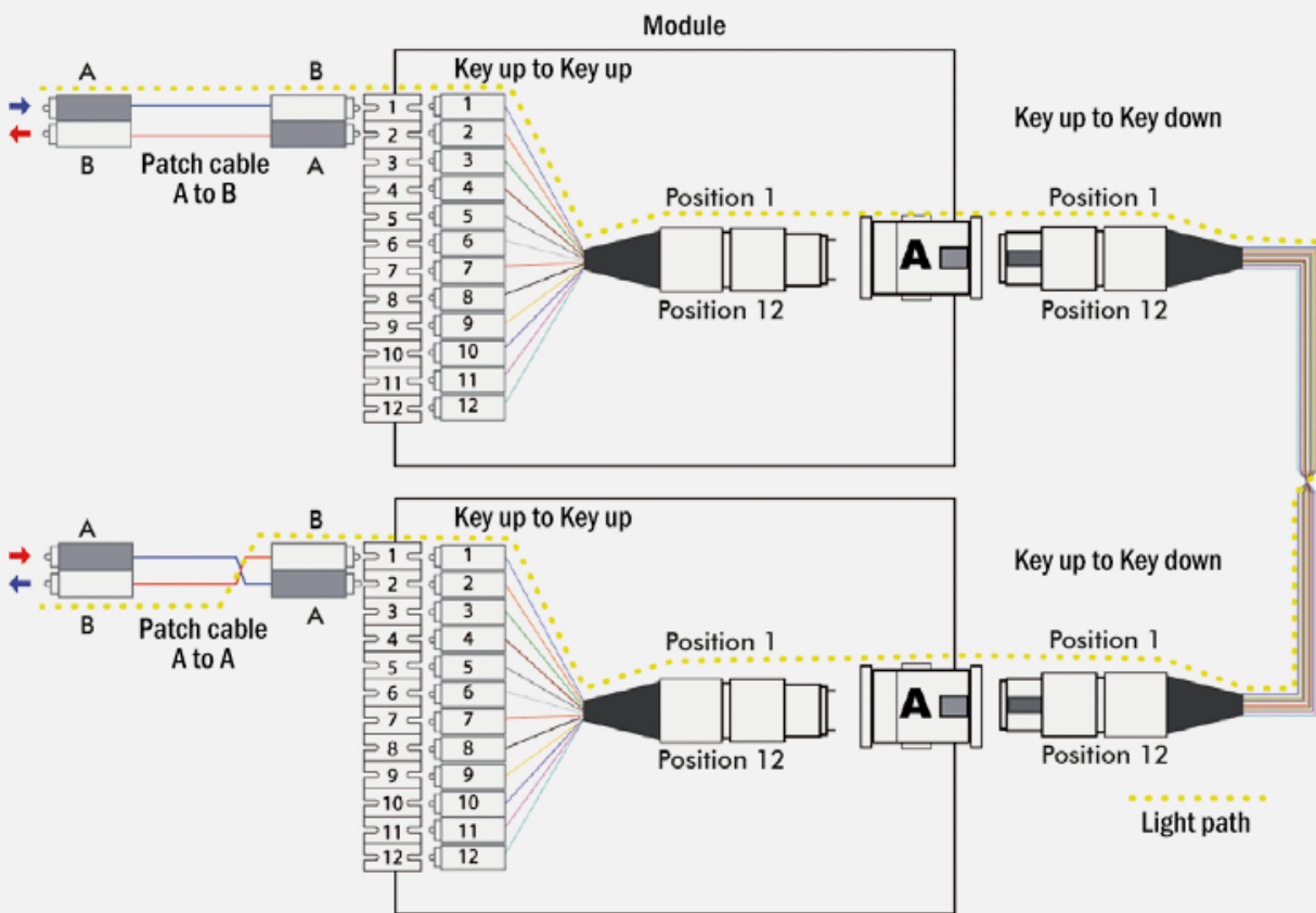
patch cable A on B
