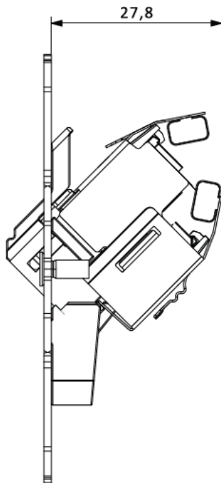
Abb.1: RJ45-TL® rapid in Anschlussdose (Art.-Nr.:127137)
